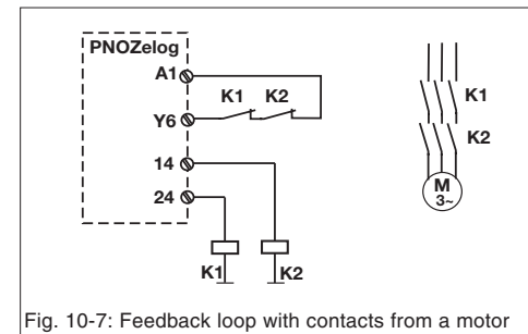
Fig. 10-7: Feedback loop with contacts from a motor
