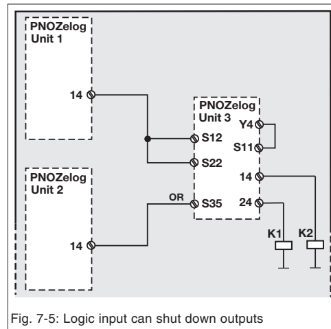
Fig. 7-5: Logic input can shut down outputs
