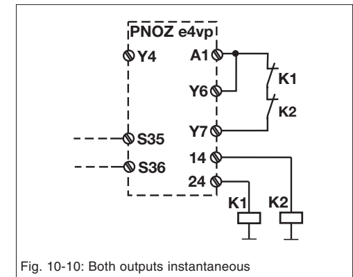
Fig. 10-10: Both outputs instantaneous
