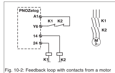
Fig. 10-2: Feedback loop with contacts from a motor
