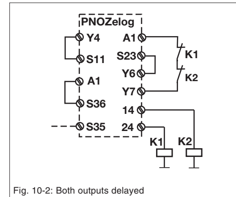
Fig. 10-2: Both outputs delayed
